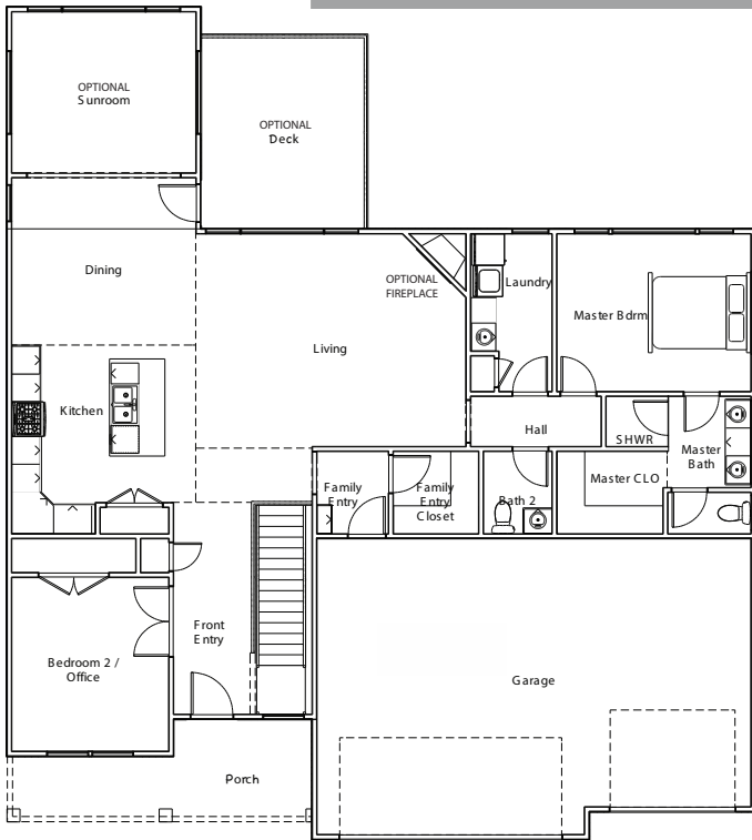
MAIN LEVEL
